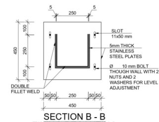
SECTION B - B FIXING DECANTING TROUGH TO END WALL
