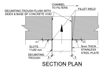
SECTION PLAN
