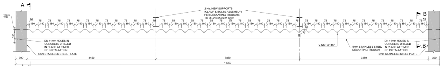
DECANTING TROUGH DETAIL
