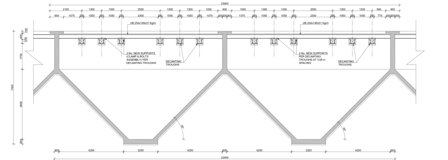
TYPICAL SECTION THROUGH SEDIMENTATION BASIN
