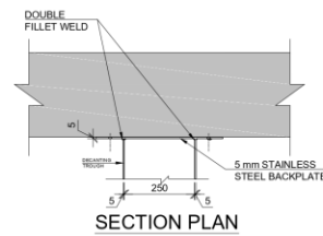
SECTION PLAN
