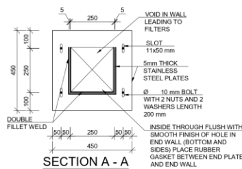
SECTION A - A FIXING DECANTING TROUGH TO FILTERS CHANNEL (ADJUSTABLE)
