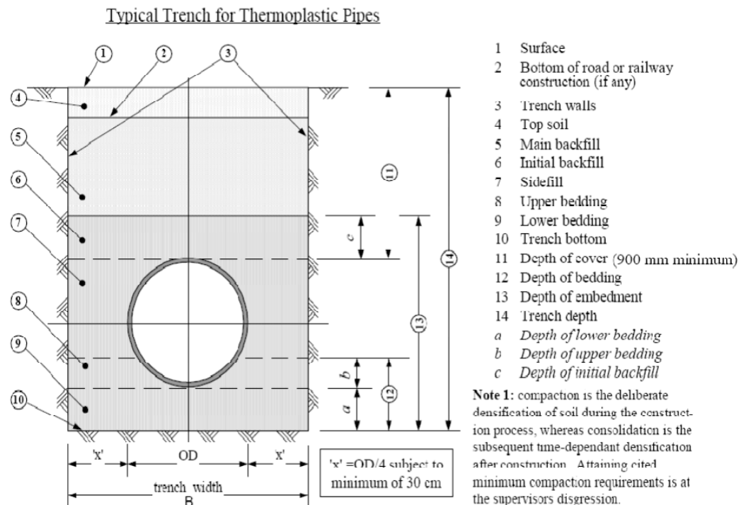
Figure: Trench Installation
