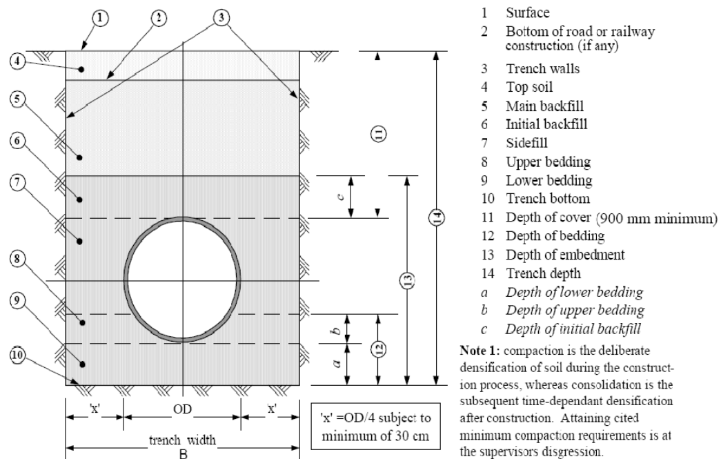
Typical Trench for Thermoplastic Pipes
